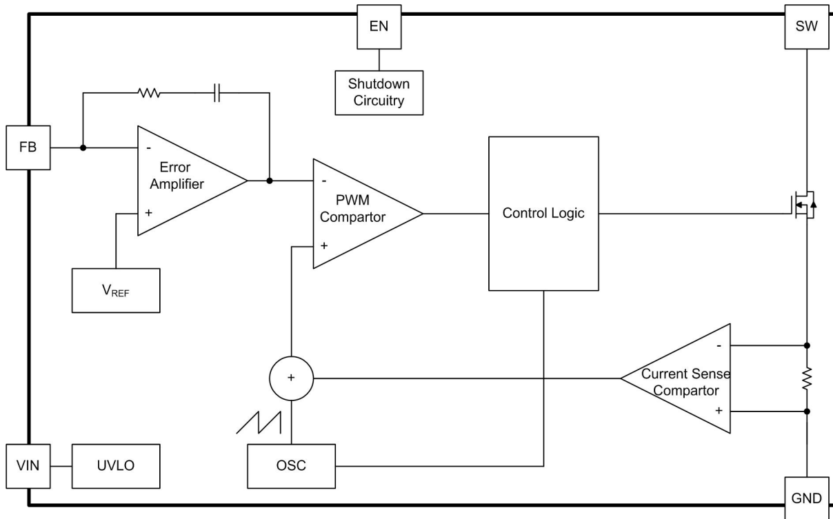
Figure 1. EC9710 Block Diagram
