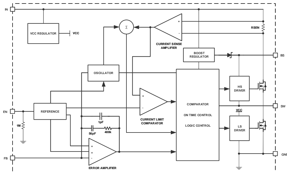
Figure 2. EC3830 Block Diagram
