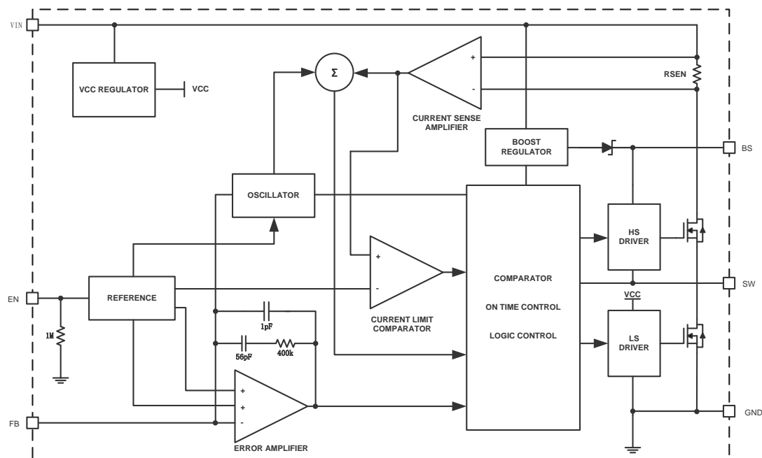
Figure 2. EC 3820 Block Diagram
