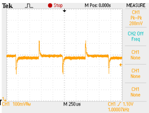
LOAD TRANSIENT RESPONSE (VIN=5V, VOUT=3.3V, IOUT=100-1400mA, 1A/μs)
