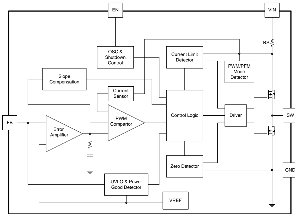
Figure 1. EC3410 Block Diagram
